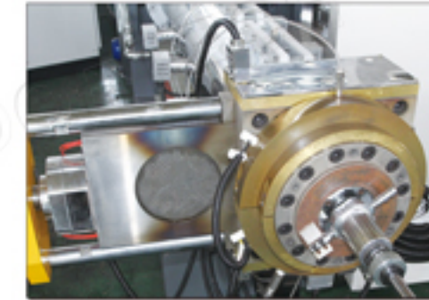
Hydraulic Screen Changer 液压换网
